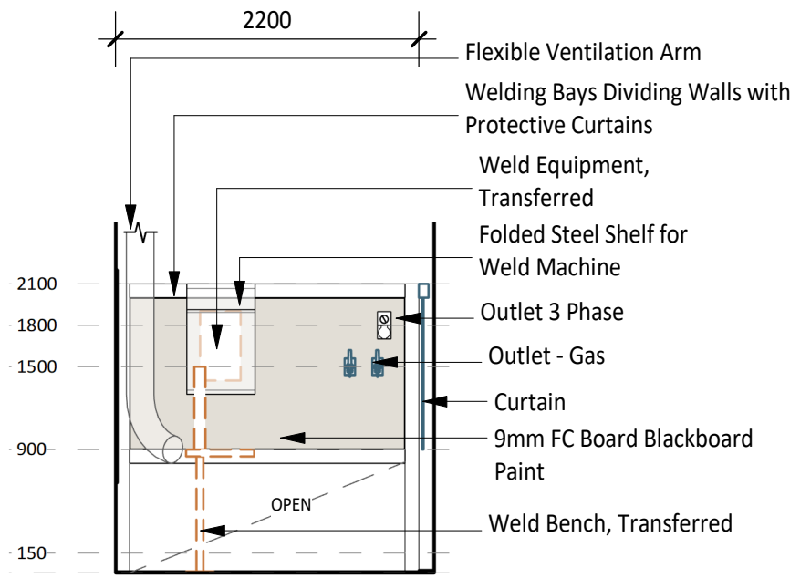
3 ELEVATION DETAIL 60-023 1 : 50
