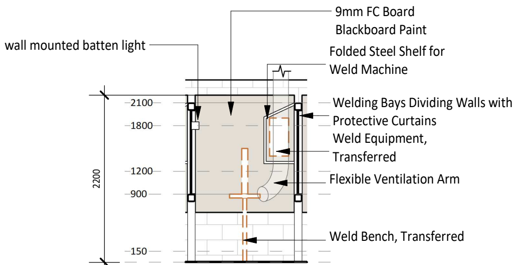
2 ELEVATION DETAIL 60-023 1 : 50
