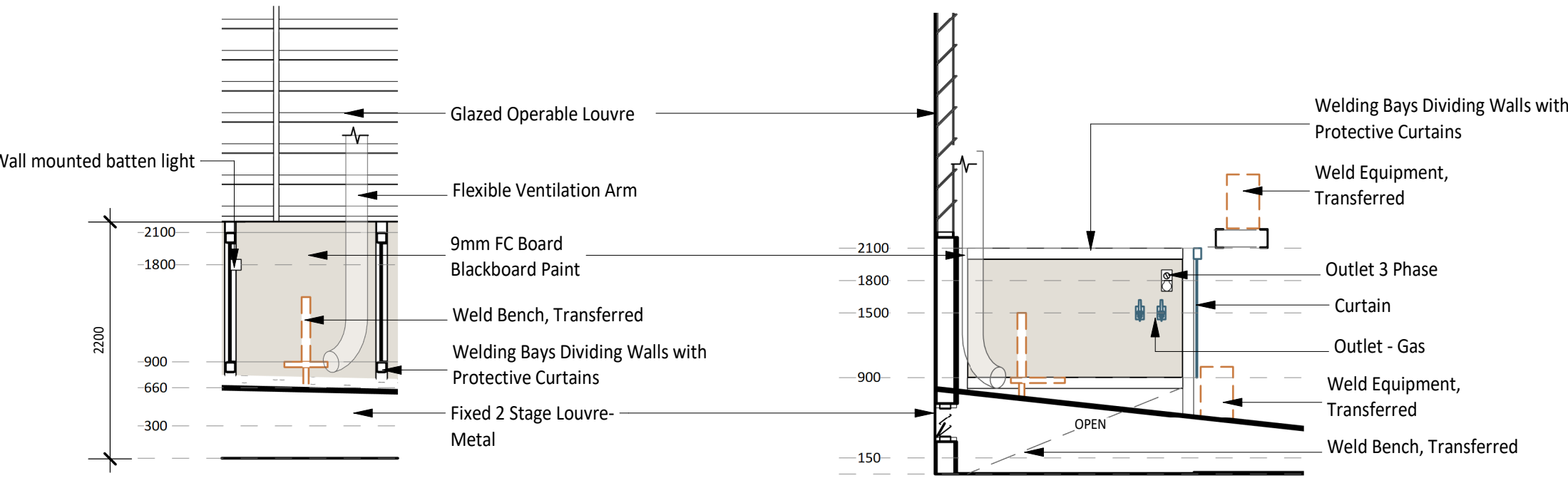
5 ELEVATION DETAIL 60-023 1 : 50
