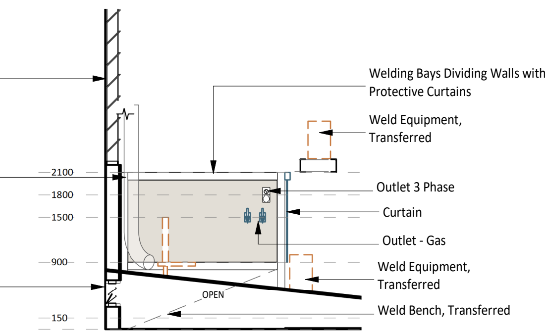
6 ELEVATION DETAIL 60-023 1 : 50
